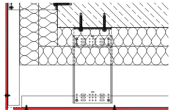
Connection to rising parts of building
