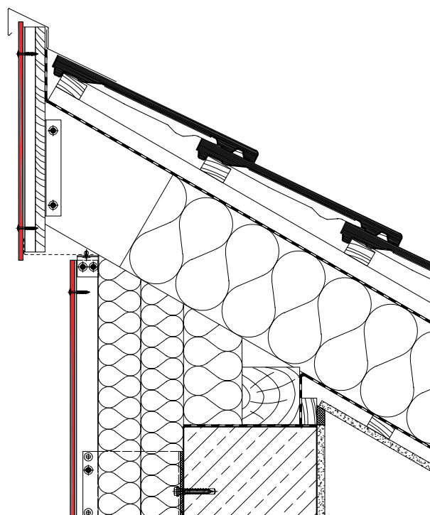
Roof ridge
