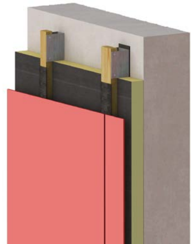
Structure with wall mounts
