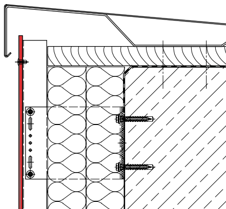
Attic connection
