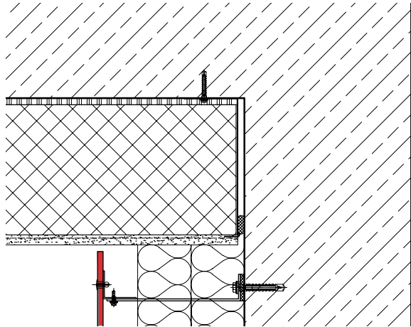
Internal Corner
