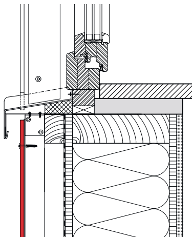
Window sill
