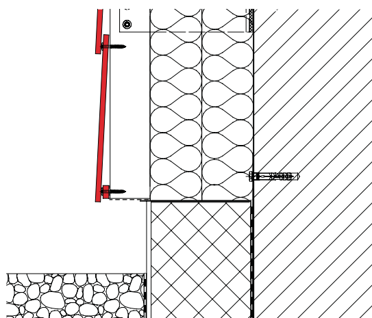
Base connection
