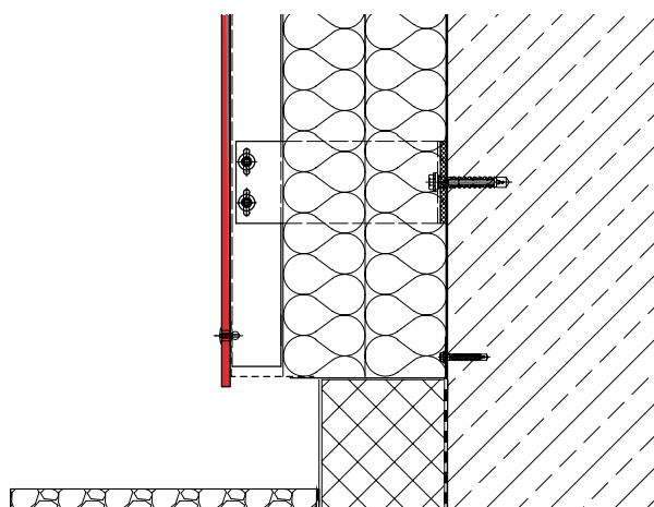
Base connection
