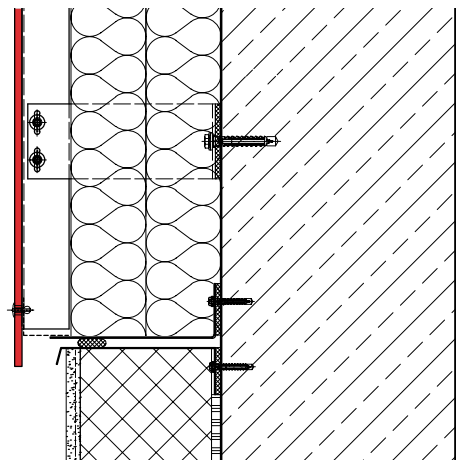
Vertical transition, RESOPLAN above
