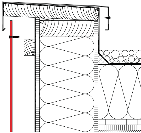
Attic connection
