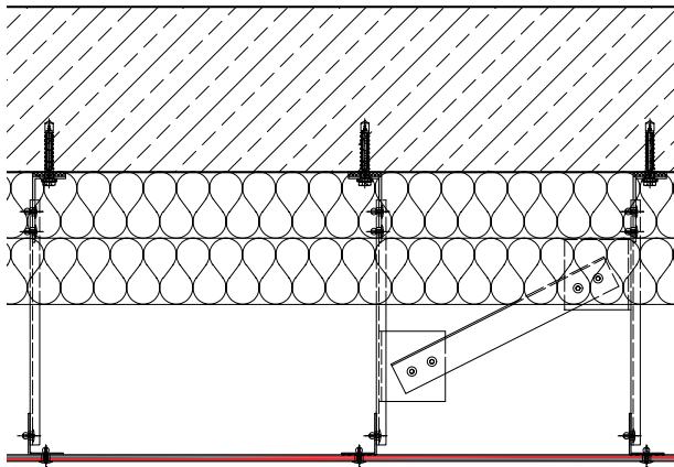
Adjustment range
