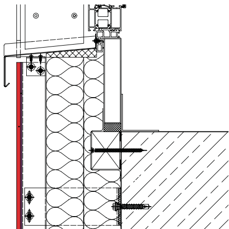
Window sill
