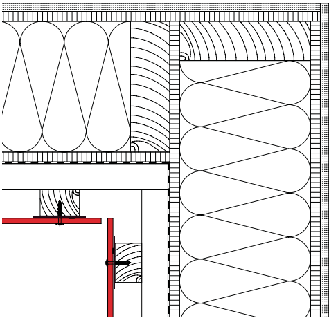
Internal corner
