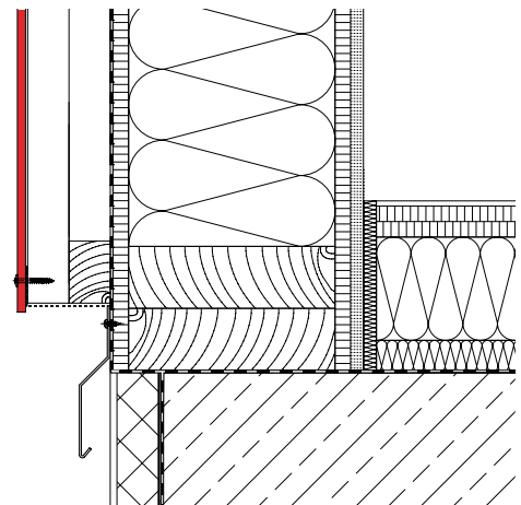
Base connection
