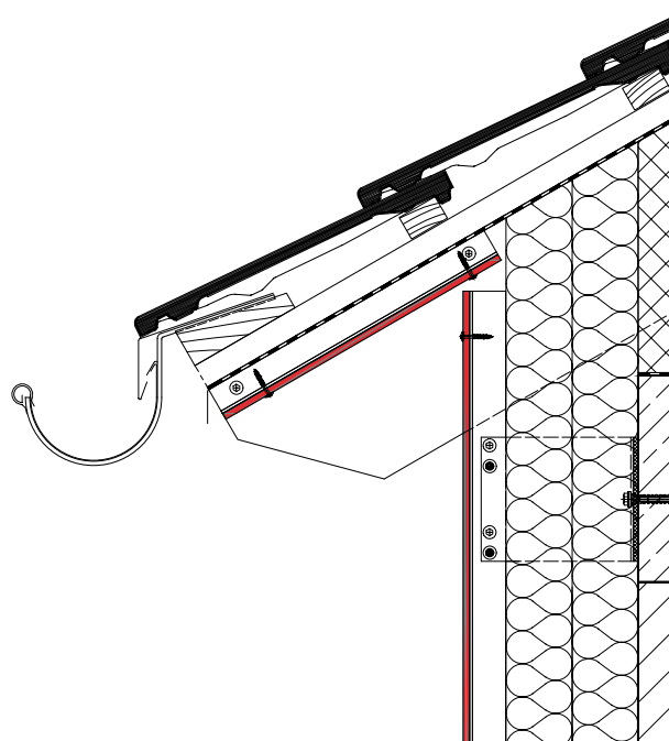
Eaves, rafters visible
