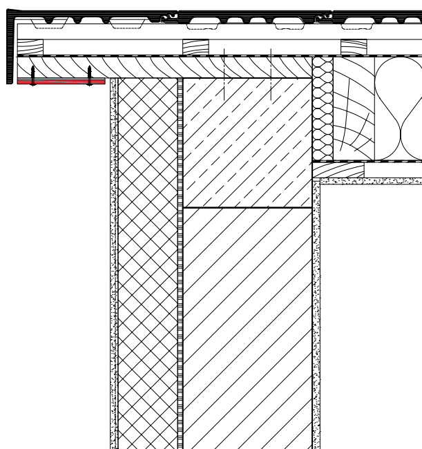
Roof overhang
