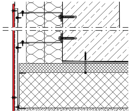
External Corner
