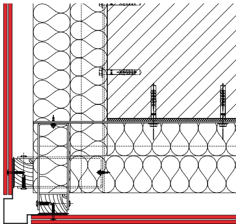
External corner
