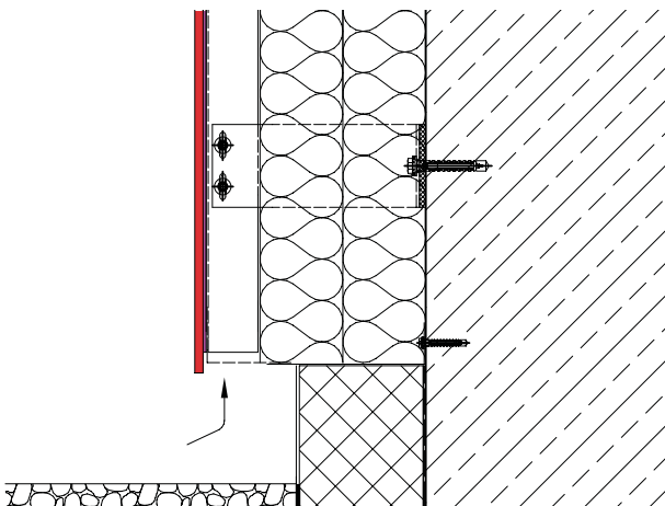
Base connection
