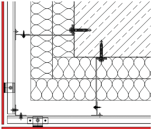
External corner
